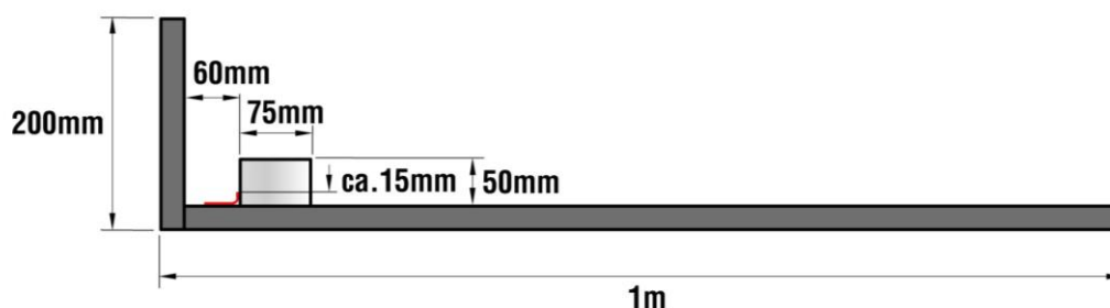
Figur 2. Testboxens dimensioner.
