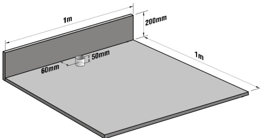
Figur 1. Testboxens dimensioner.
